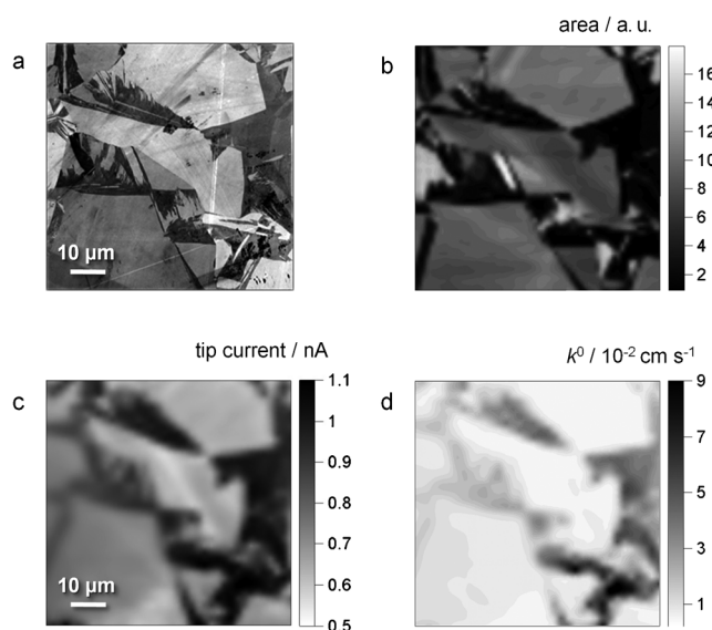
Figure 1. Images ( 70\ \mu\text{m} \times 70\ \mu\text{m} ) of pBDD obtained using a) FE-SEM recorded with an in-lens detector at 2 kV. b) Raman mapping, showing the integrated peak area at about 1332\ \text{cm}^{-1} as a function of spot position. c) IC-SECM SG-TC map for the collection of \text{Ru}(\text{NH}_3)_6^{2+} (by oxidation), electrogenerated at the surface of pBDD ( \eta = -0.004\ \text{V} ). d) Calculated k^0 values from the currents in (c) using finite element simulations.
